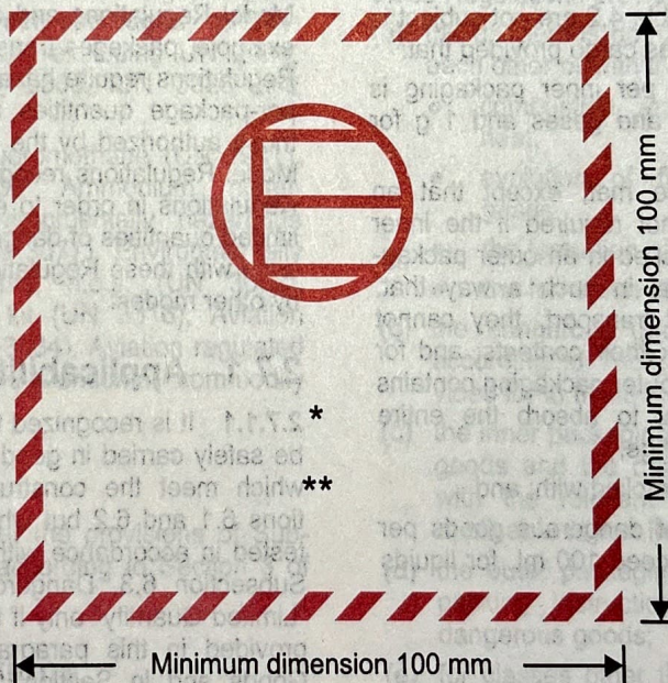
FIGURE 2.6.B Excepted Quantity Package Mark (2.6.7.1)
